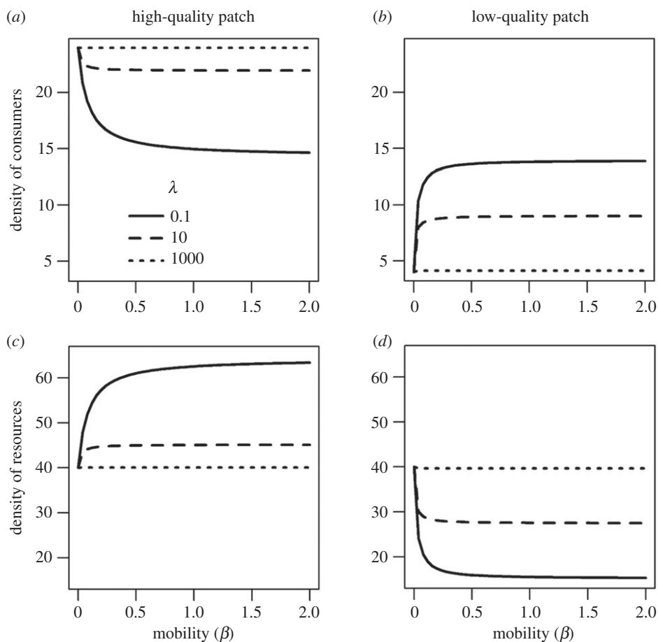
Figure 3. Relationship between equilibrium densities of consumers ( a,b ), resources ( c,d ) and mobility ( \beta ) in the high- ( a,c ) and the low-quality patch ( b,d ) in the presence of consumer demography ( p = 1 ). Fitness sensitivity is set at three levels: \lambda = 0.1, 10 and 1000. Other parameters are: r_H = 2 , r_L = 1 , K_H = 100 , K_L = 50 , c = 0.05 , \alpha = 0.05 and \mu = 0.1 .
